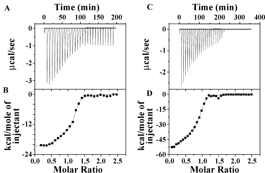
FIGURE 2: Raw isothermal titration calorimetry data and binding isotherm data for ferrous iron binding to Dfh (A and B, respectively) and holo-Dfh binding to Isu (C and D, respectively). Gray lines in panels A and C show baselines for the raw ITC data. Gray lines in panels B and D show simulated fits to binding isotherm data. Data were collected anaerobically at 30 °C in 20 mM HEPES (pH 7.0) and 10 mM \text{MgSO}_4 for ferrous iron binding to apo-Dfh and in 20 mM HEPES (pH 7.5) and 150 mM NaCl for holo-Dfh binding to Isu.
