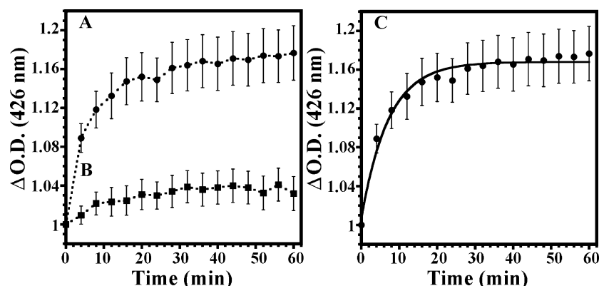
FIGURE 5: Time dependence for formation of the Fe–S cluster on ISU. The solution contained 100 \mu M Isu, 4.3 mM DTT, and 2.4 mM \text{Na}_2\text{S} in 20 mM HEPES buffer (pH 7.5), with 150 mM NaCl to which Fe(II) was added as holofrataxin (● in part A) or directly (■ in part B) to a final concentration of 100 \mu M. Reaction progress was monitored at 426 nm. (C) Time dependence data (●) from panel A fit with a rate equation for a first-order process (simulation as a solid line). Error bars represent the average values at each time point from the three independent reproducible experiments that were conducted.
