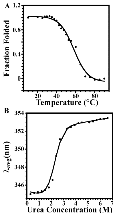
FIGURE 1: Representative thermal (A) and chemical (B) denaturation profiles for apo-Dfh. In both spectra, dots represent raw data while the line represents the spectral simulation. The thermal denaturation curve for Dfh was determined by measuring changes in molar ellipticity at 208 nm from the protein's CD spectra taken at multiple temperatures. The urea denaturation curve for Dfh followed a red shift in fluorescence; spectral simulation from reproducible data sets provided the following stability parameters: [\text{urea}]_{50\%} = 2.37 \pm 0.23 M, \Delta G^{\text{H}_2\text{O}} = 7.44 \pm 0.47 kcal/mol, and m = 3.13 \pm 0.20 kcal mol -1 M -1 .
