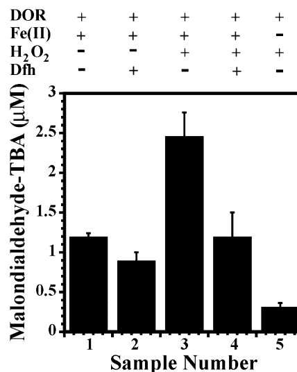
FIGURE 3: Oxidative degradation assay. Reaction mixtures were incubated in the presence or absence of Dfh [in 20 mM HEPES (pH 7) and 10 mM \text{MgSO}_4 ] to test the ability of Dfh to attenuate oxidative degradation of 2-deoxyribose sugars to produce malondialdehyde.
